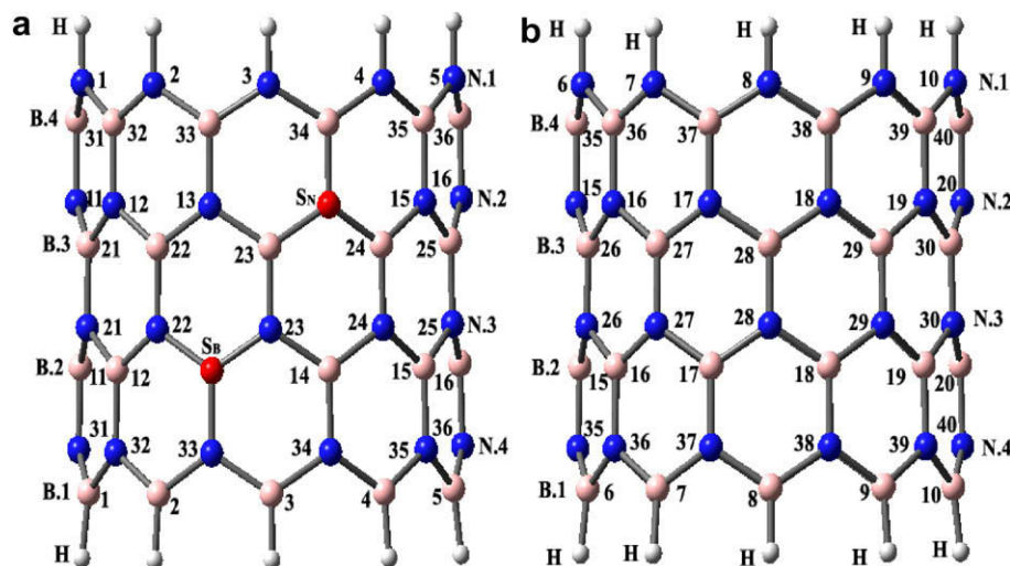
Figure 2 The schematic diagram of boron-nitride nanotube (10, 0), magenta and blue spheres are boron and nitrogen atoms, respectively. Two substitutional sites S_B and S_N (red spheres) for carbon, silicon and germanium atoms. (a) The front side and (b) the back side.
