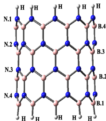
Figure 1 The 2D view of the pristine (10, 0) BN nanotube.
