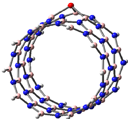
Figure 3 The 3D view of Ge-substituted ( S_N ) (10, 0) BNNT.
